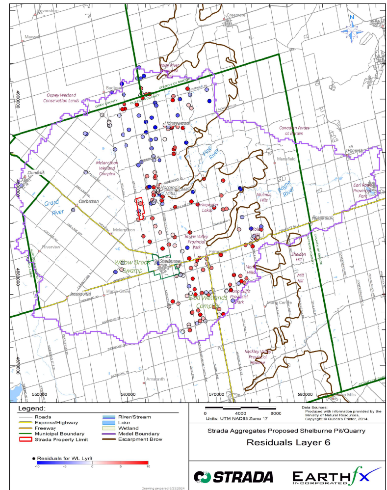
Figure 4.14: Observed-simulated residuals in the Gasport Formation.
