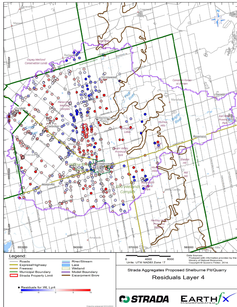
Figure 4.13: Observed-simulated residuals in the Guelph Formation.
